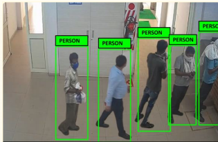
Queue Detection
