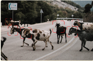
Animal Detection
